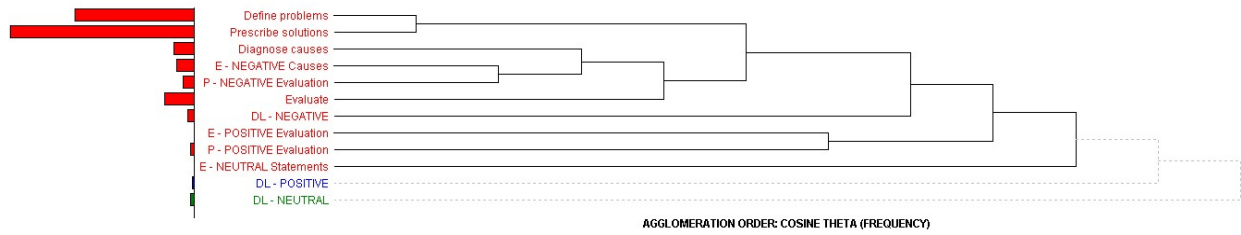
Figure 5. Cluster analysis
